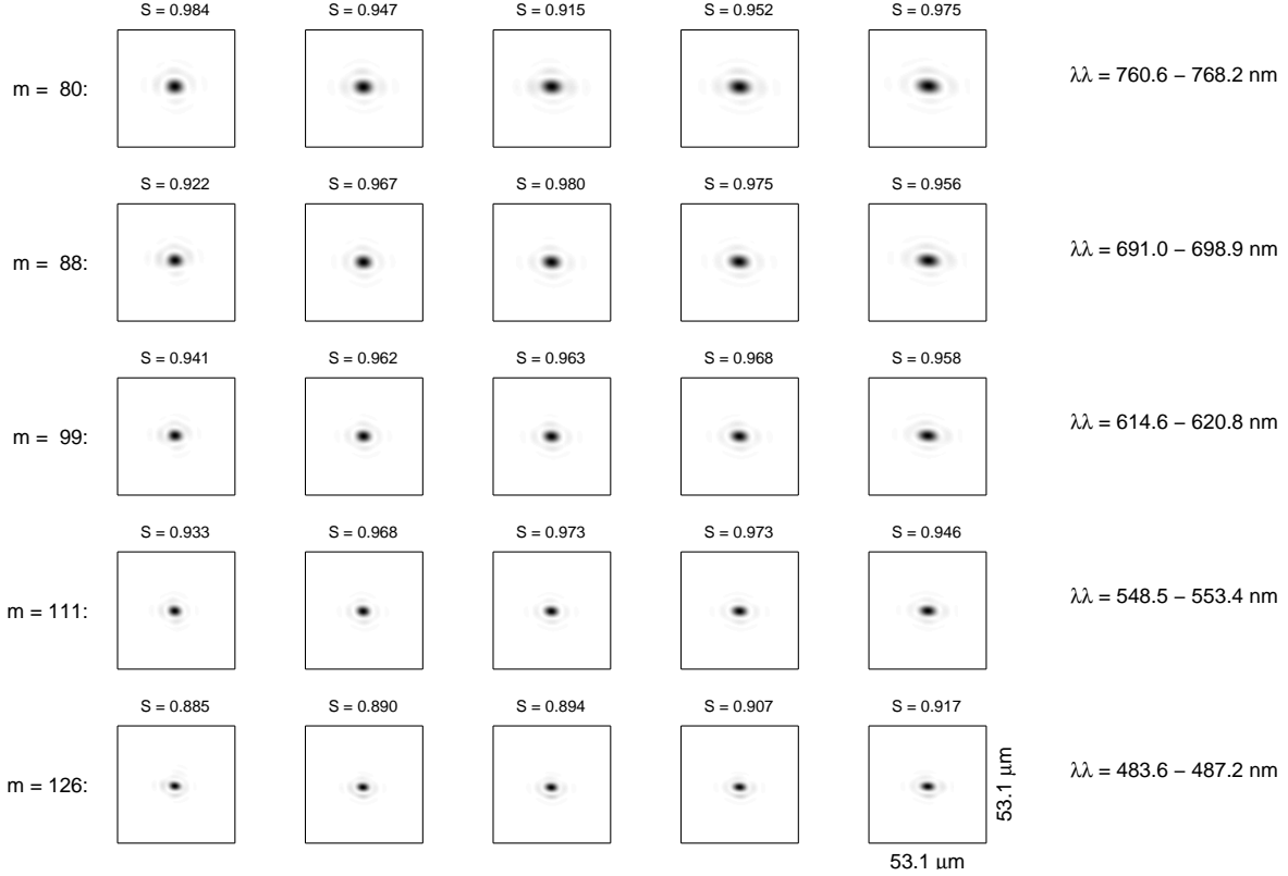
Figure 5. Image quality of the preliminary WISDOM green channel camera. The point source PSF images uniformly cover the spectral format in this channel (see Fig. 6). Each box is one resolution element (3.5 pixels) square. The Strehl ratio ( S ) is shown above each box. See Fig. 4 for the corresponding spot diagrams.
